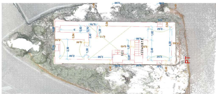
Figure 12. Combination of geometric data from the external and internal surveys.
